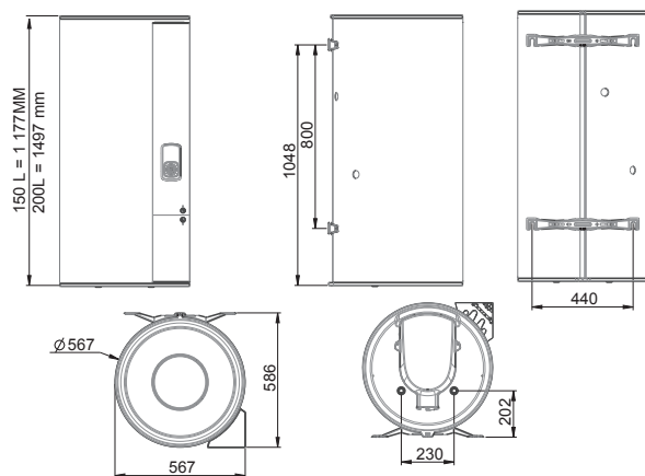
Vertical mural 150 L et vertical mural 200 L
